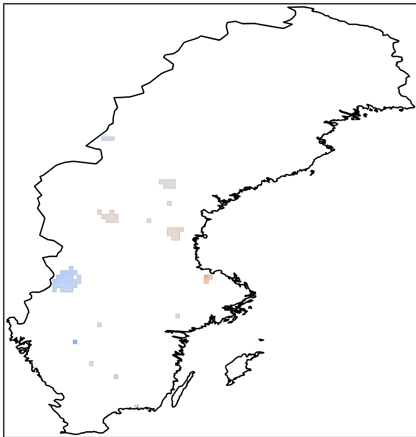
Heatwave index and groundwater levels
